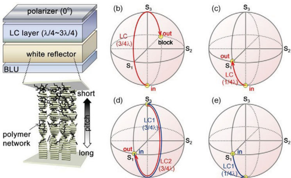
Figure 3. (a) Schematic diagram and (b)-(d) polarization representations of our proposed transfective LC display consisting of the nematic LC display as a conventional light modulator and the cholesteric white reflector as a transfective mirror. Optical pathways for (b) dark and (c) bright states in the transmissive mode, and for the (d) bright and (e) dark states in the reflective mode represented on the Poincaré Sphere.
