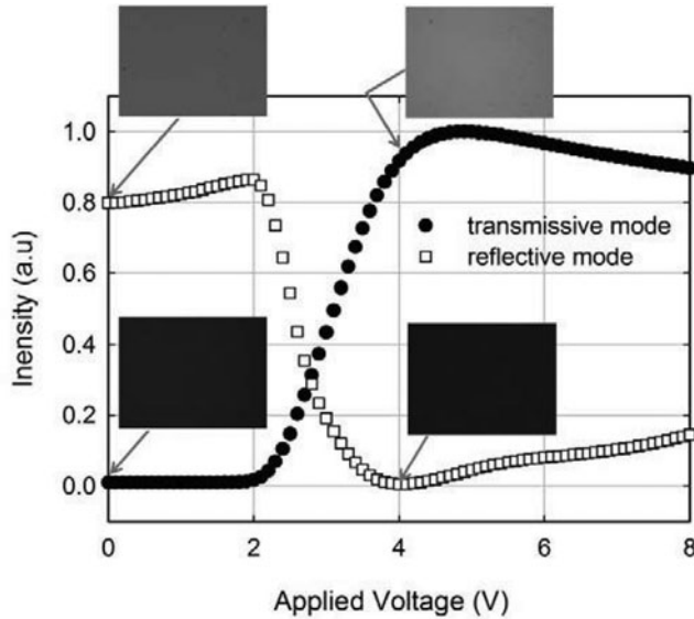
Figure 4. Measured electrooptic properties and corresponding microscopic textures in both transmissive and reflective modes.
