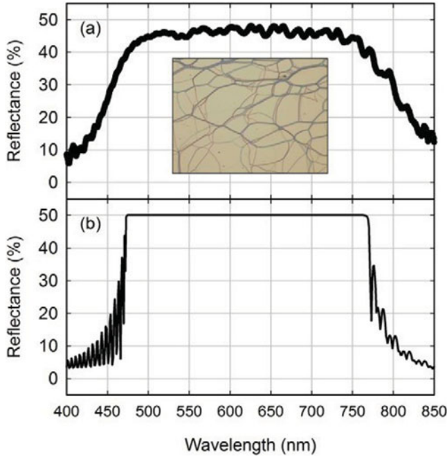
Figure 2. (a) Measured and (b) calculated spectra of reflection from the cholesteric white reflector. Inset image represents the reflected microscopic texture.
