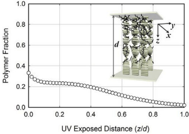
Figure 1. The volume fraction of the RM polymer with chirality and schematic diagram as function of the distance from UV illuminated surface.
